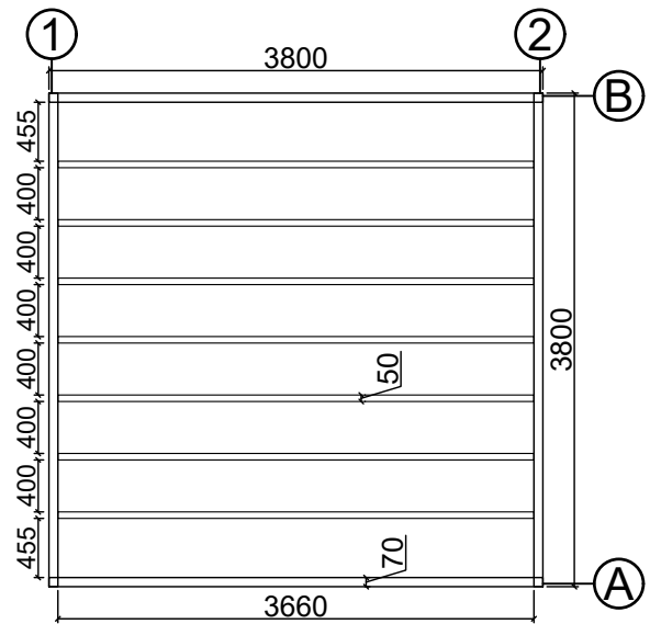
Base plan
