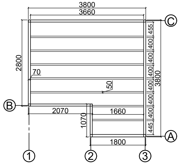
Base plan
