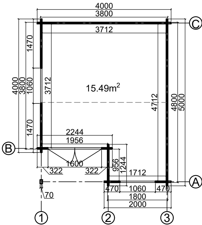
Floor plan
