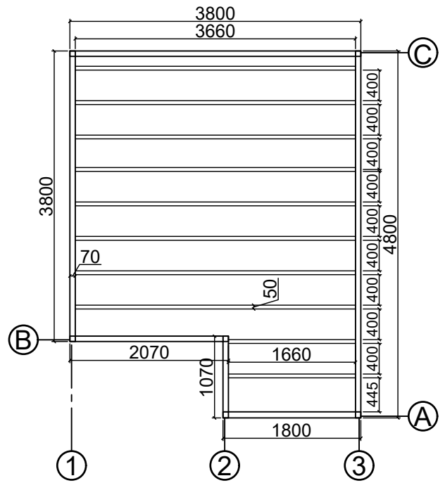
Base plan
