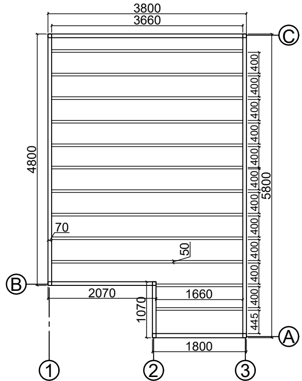
Base plan
