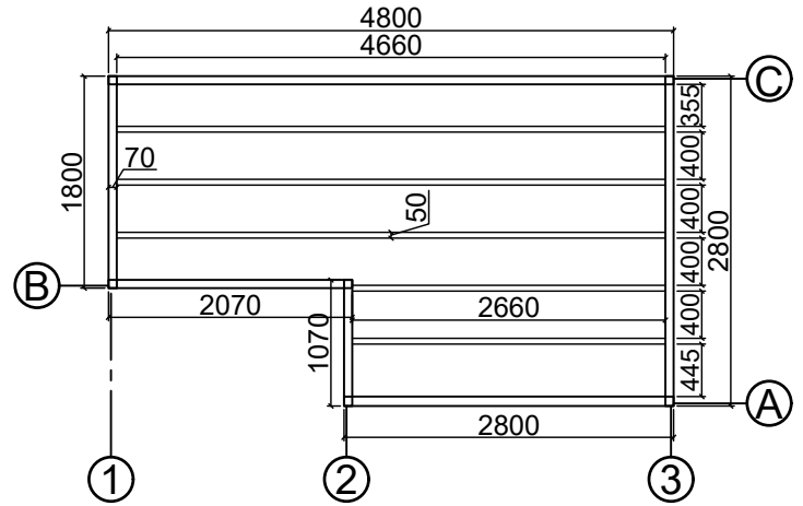
Base plan
