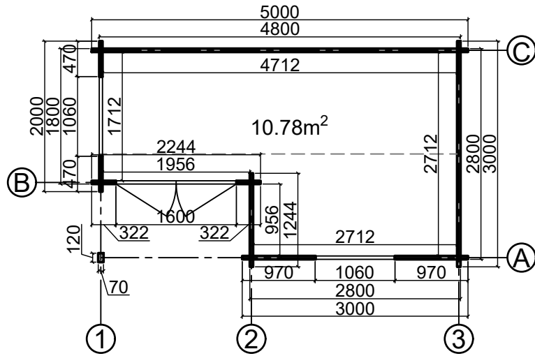
Floor plan
