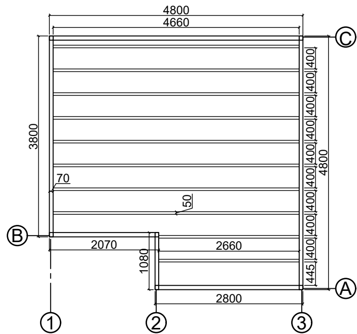
Base plan
