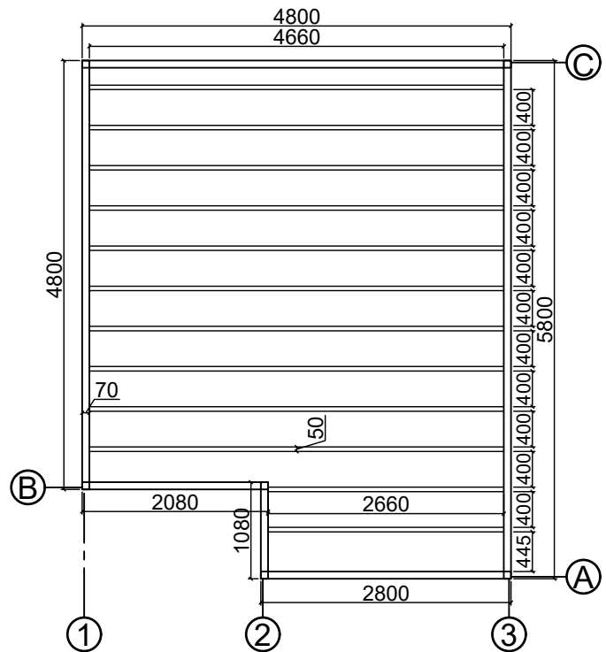
Base plan
