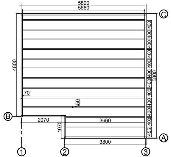
Base plan
