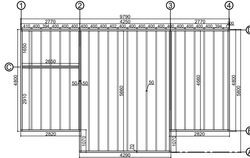
Base plan
