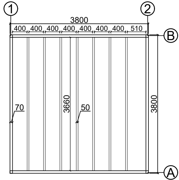
Base plan
