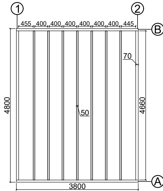
Base plan
