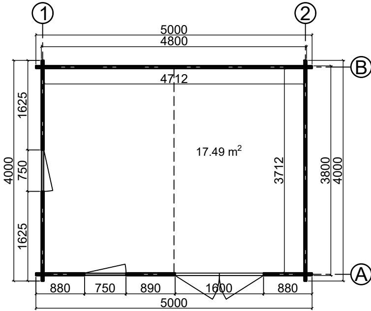
Floor plan
