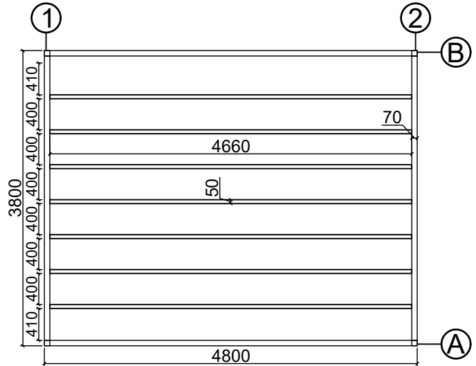
Base plan
