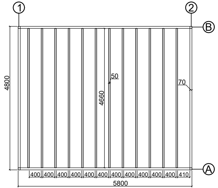
Base plan
