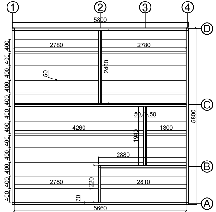
Base plan
