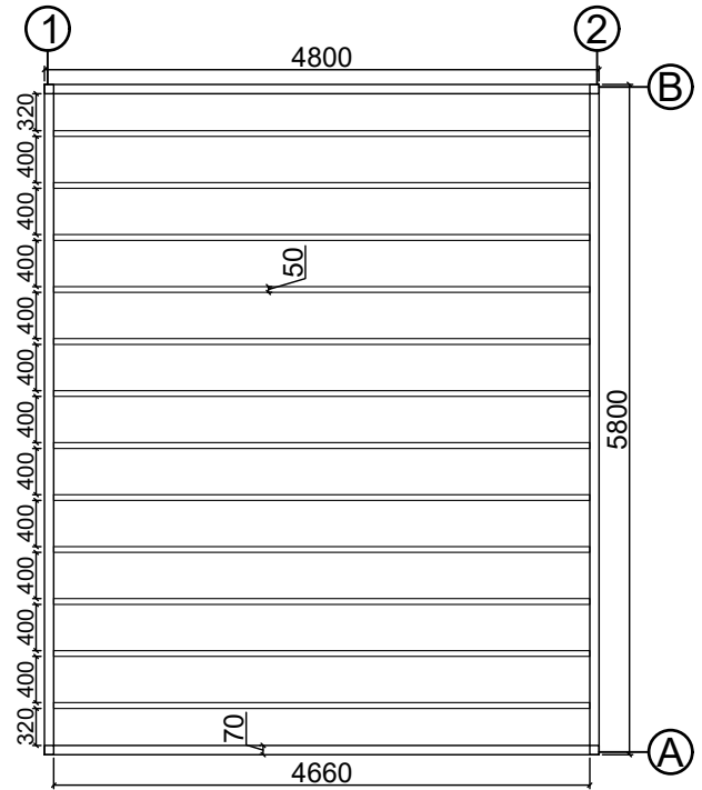
Base plan
