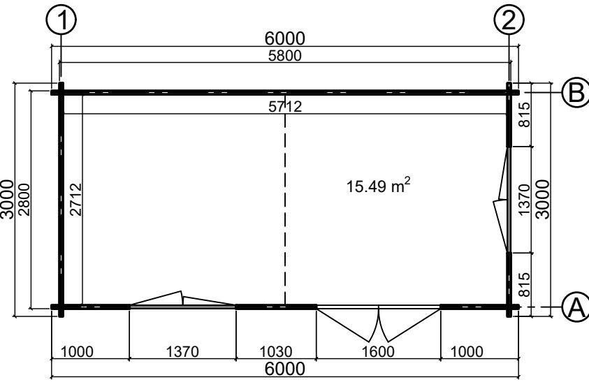
Floor plan
